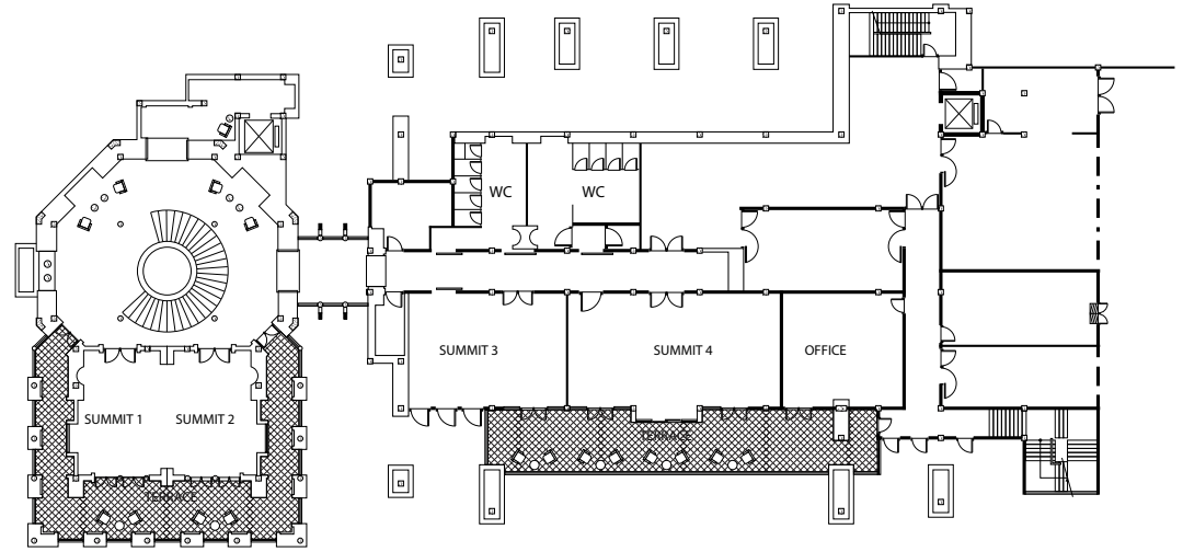
THE SUMMIT GROUND FLOOR
