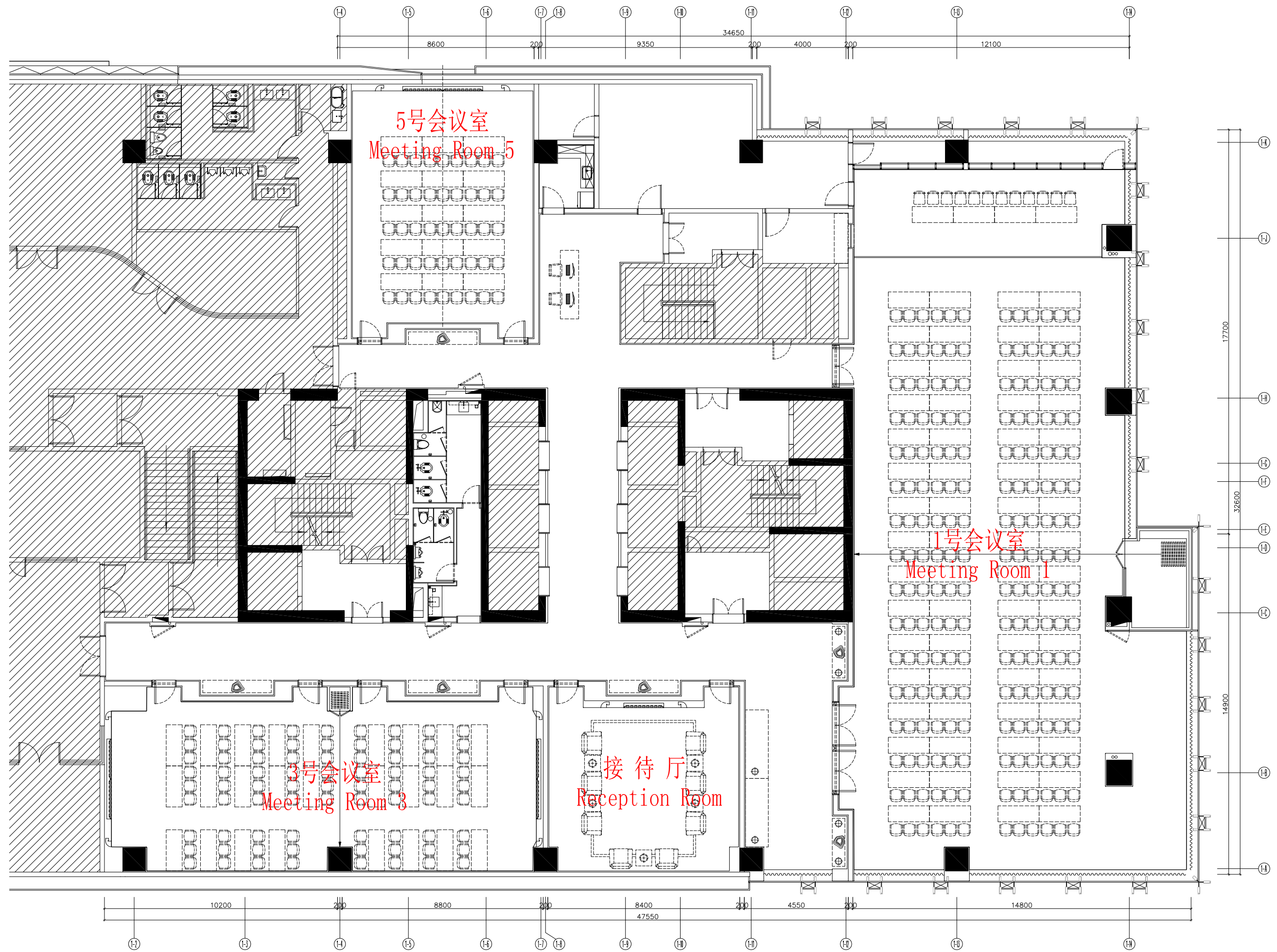
会议中心平面布置 Meeting Room Floor Plan
